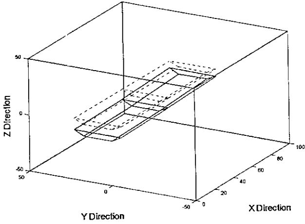
FDD Mode Shape - mode # 1, f = 0.17391 Hz, z = 1.0871 %
