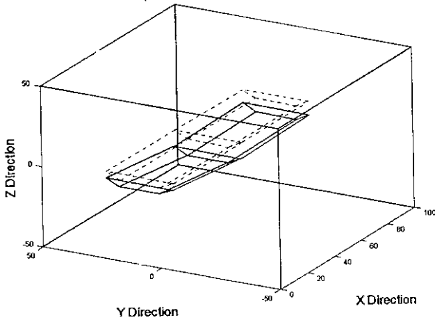
FDD Mode Shape - mode # 3, f = 0.23837 Hz, z = 0.5365 %
