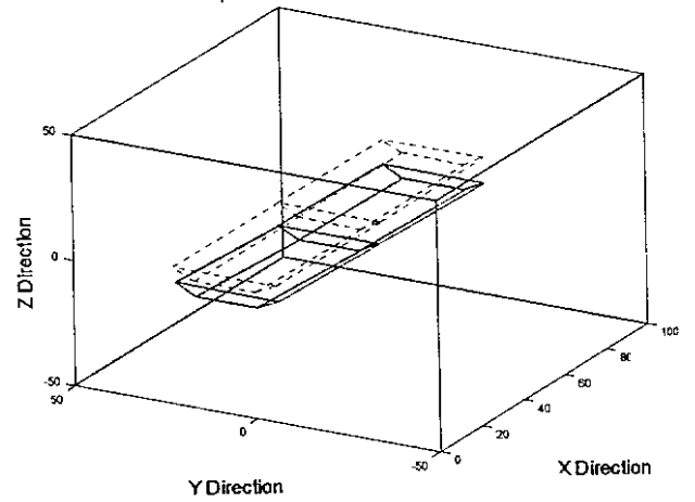
SSI Mode Shape - mode # 2, f = 0.20809 Hz, z = 0.82606 %
