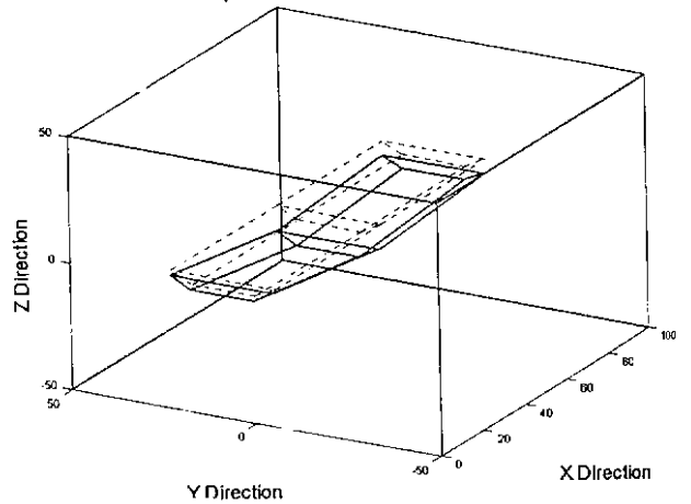
SSI Mode Shape - mode # 3, f = 0.23593 Hz, z = 6.4146 %
