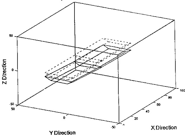
FDD Mode Shape - mode # 2, f = 0.2077 Hz, z = 0.57873 %
