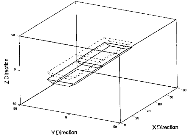
SSI Mode Shape - mode # 1, f = 0.17246 Hz, z = 0.41761 %
