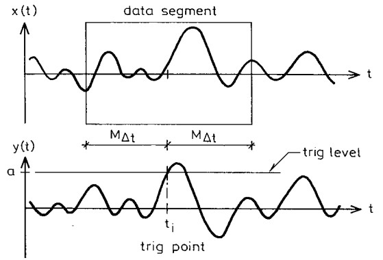
Figure 1. The Random Decrement technique.
