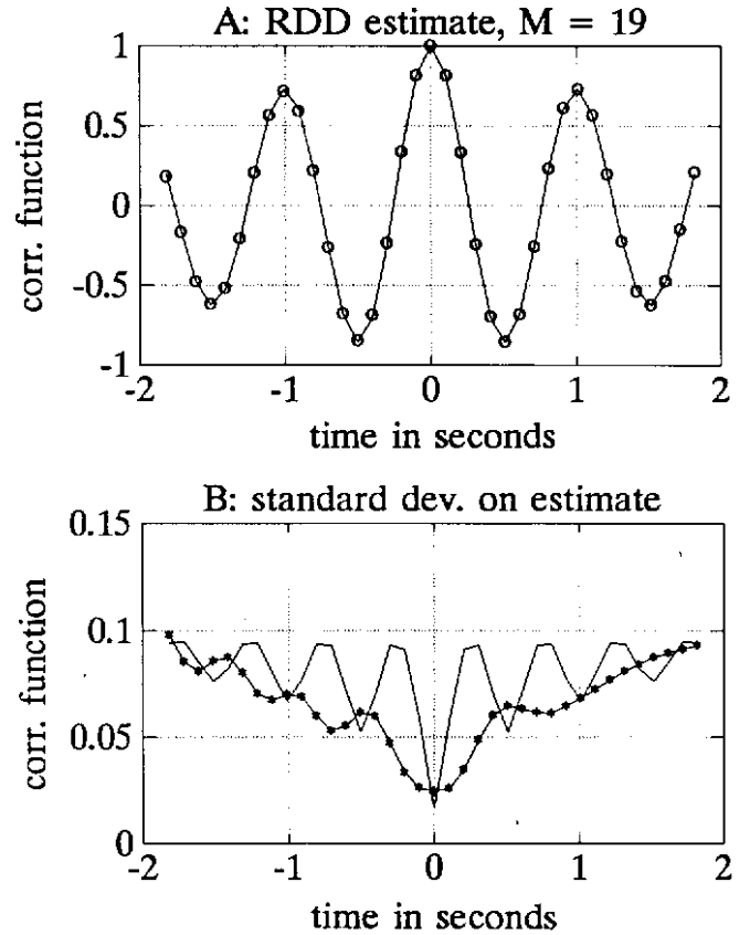
Figure 4. Estimation of auto correlation function. A: comparison between Random Decrement estimate ("o") and exact solution ("-") and B: between theoretical ("-") and empirical ("*") standard deviation.
