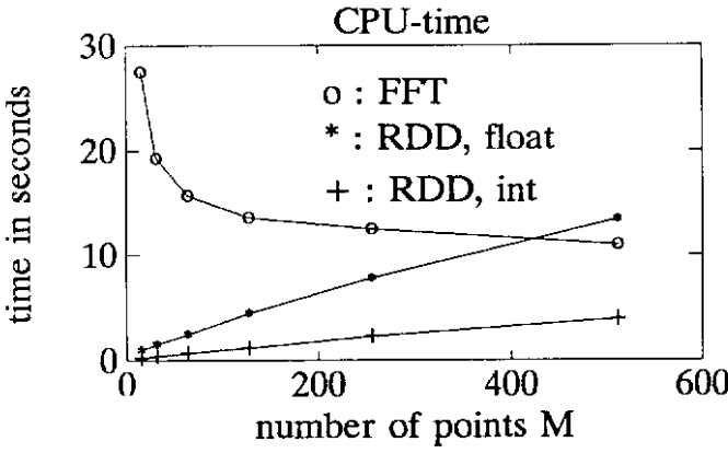
Figure 5. Comparization of CPU times for Fast Fourier Transform and Random Decrement on a time series of 4000 data points.
